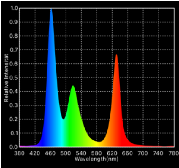
wavelengths RGB
